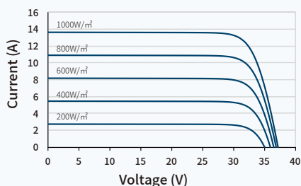
Current-Voltage (450W)
