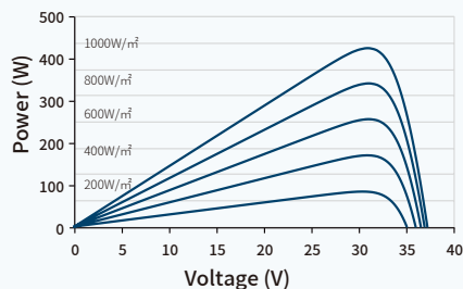
Power-Voltage (450W)
