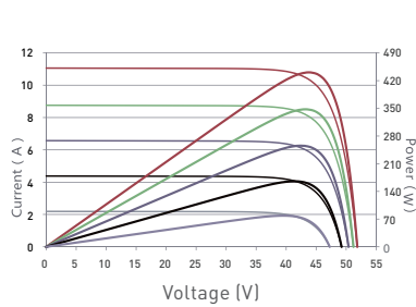
Current-Voltage & Power-Voltage Curves (475W)
