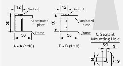
Cross Section A-A & B-B
