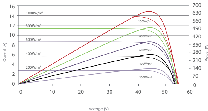
Current-Voltage & Power-Voltage Curves (640W)
